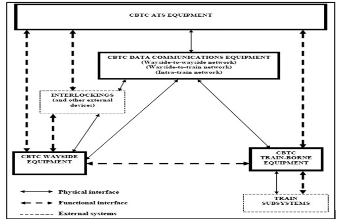
Figure 4. CBTC Subsystems.
