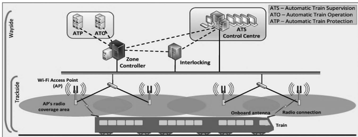
Figure 5. CBTC equipment [32].
