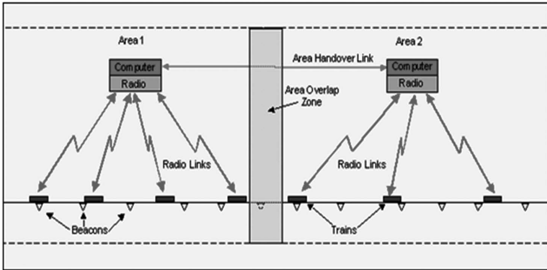
Figure 6. CBTC system.
