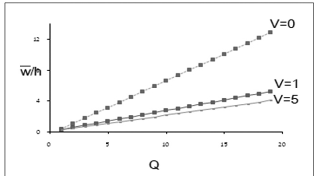
Figure 4(b). Presence of shear layer influence the flexural behaviour under various Q values, for circular panels of SS edge.
